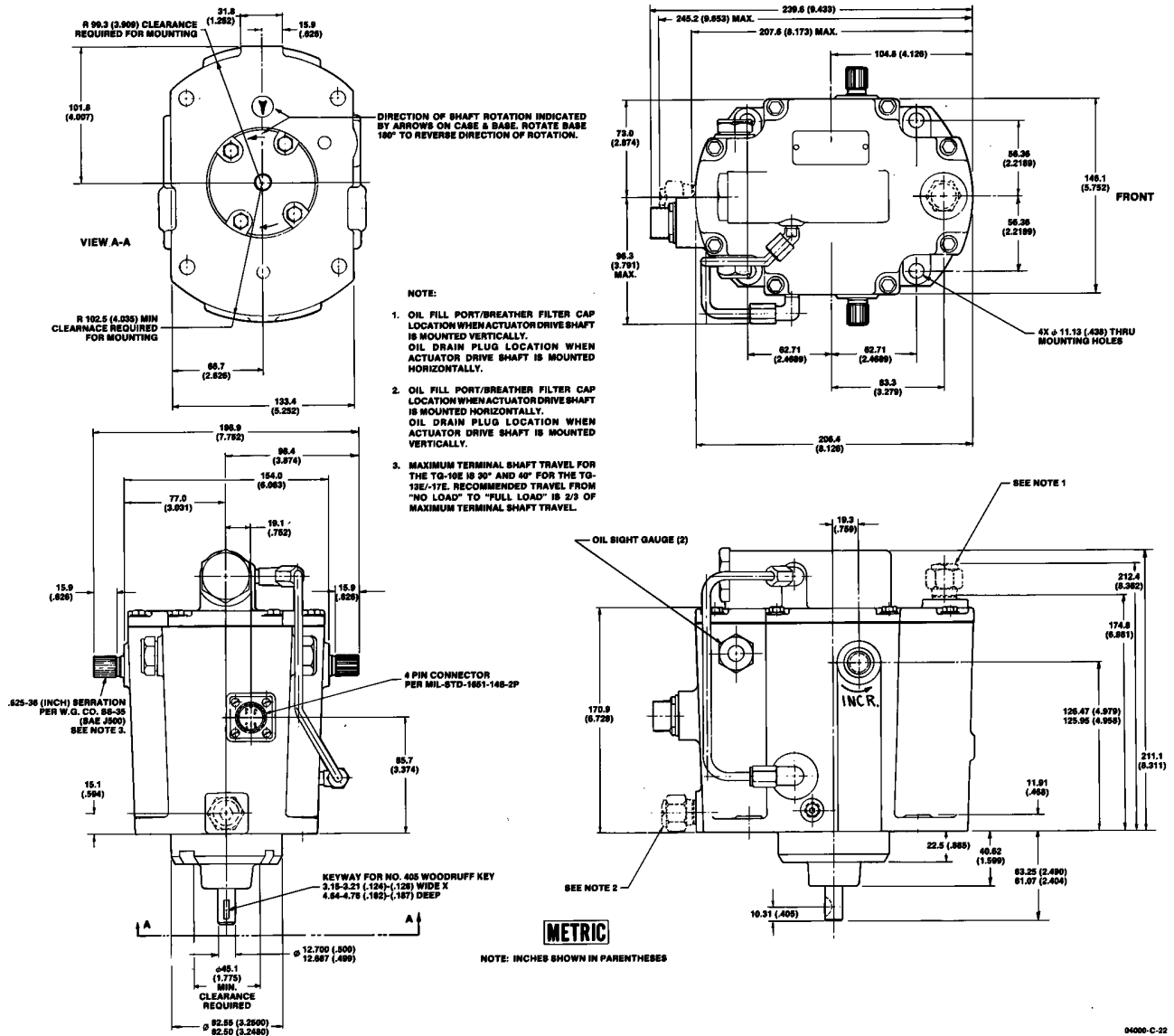
Figure 1. Outline Drawing of TG-13E and TG-17E (Do not use for construction)
