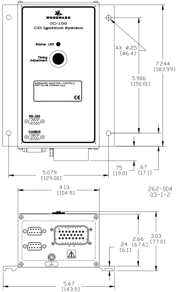
IC-100 Ignition System (Do not use for construction)
