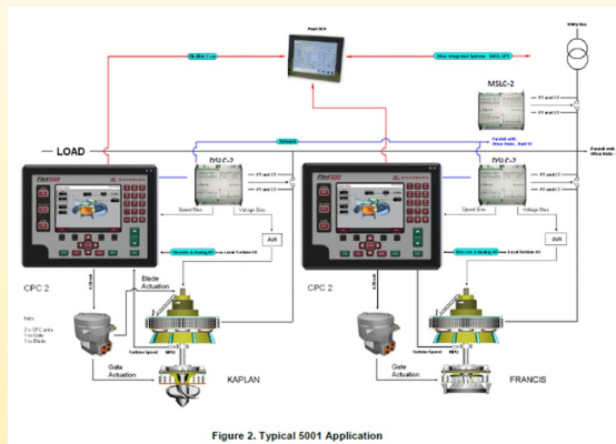
Figure 2. Typical 5001 Application
